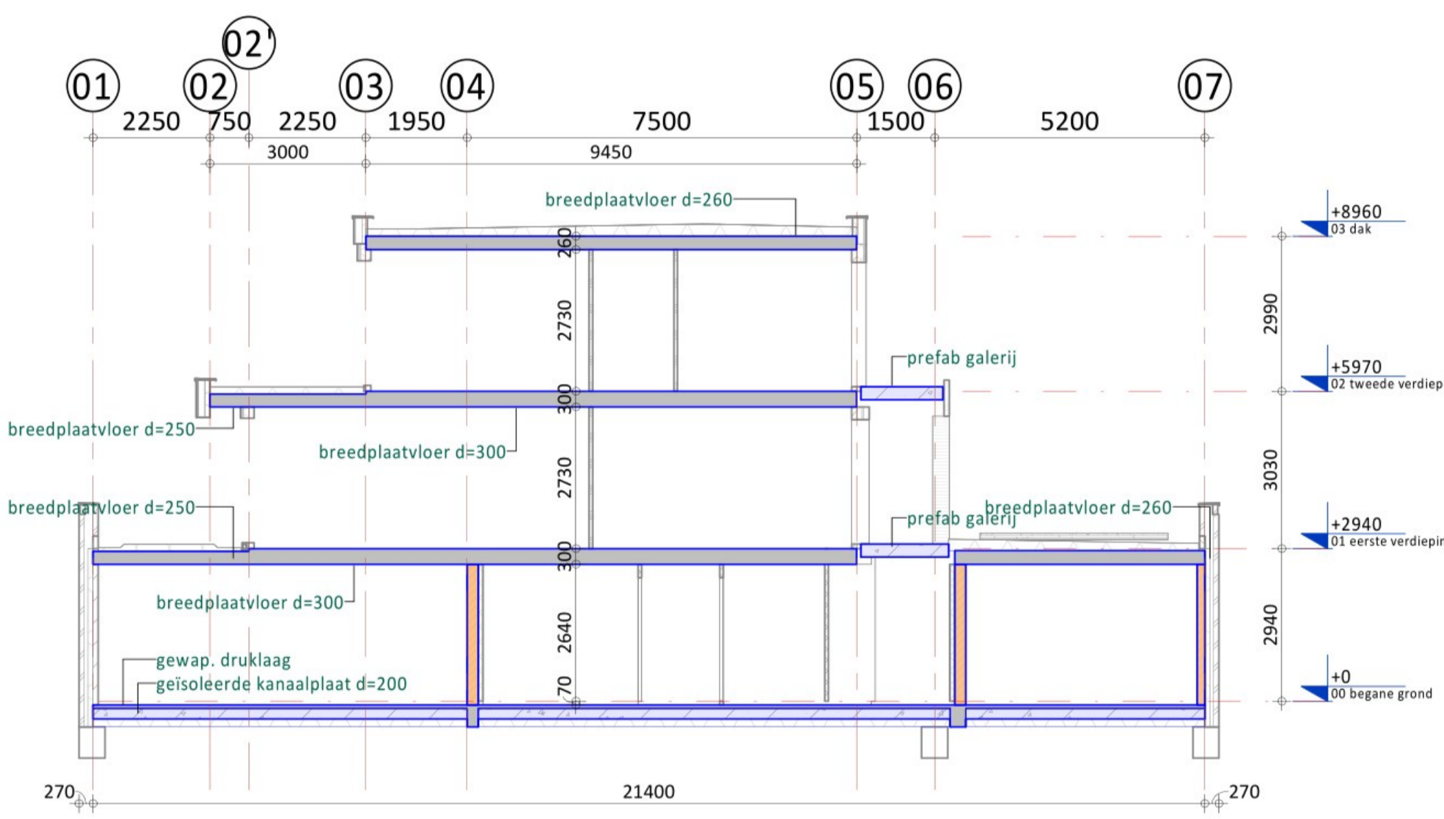
Drasn. E-E
