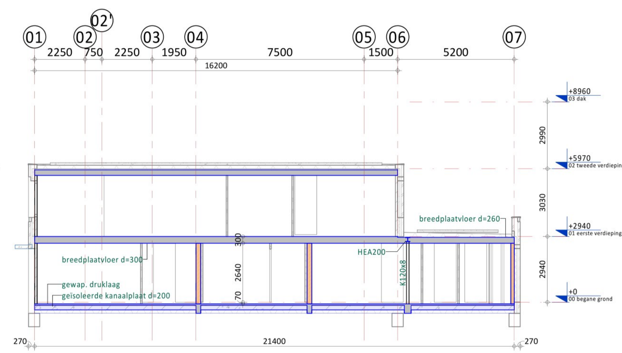
Drasn. F-F
